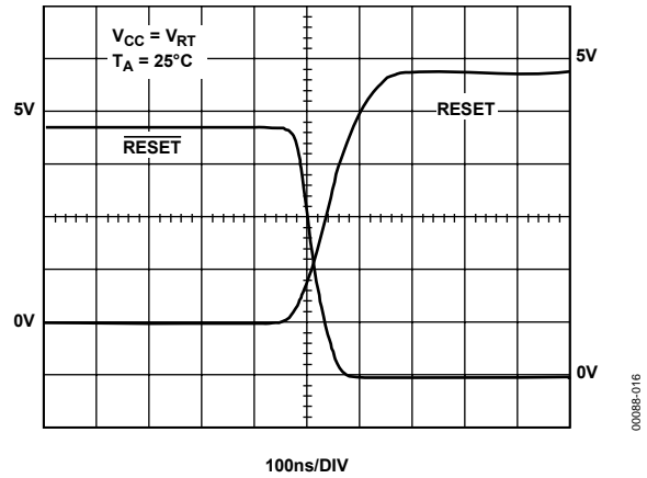
Figure 9. \overline{\text{RESET}} , \overline{\text{RESET}} Assertion
