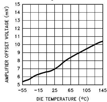
Amplifier Offset Voltage vs Die Temperature
