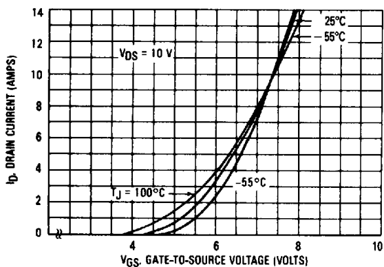
Figure 3. Transfer Characteristics
