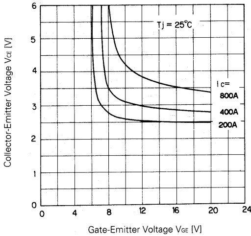
Collector-Emittor Voltage vs. Gate-Emittor Voltage
