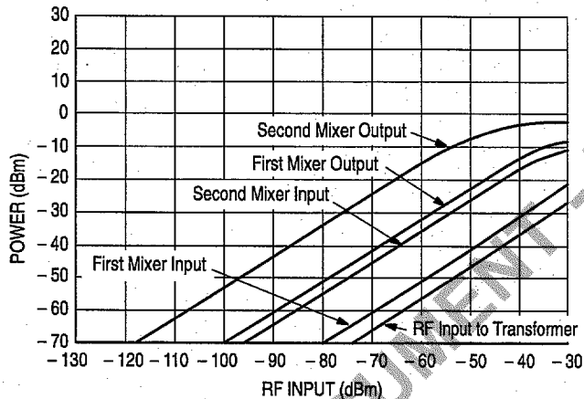
Figure 6. Signal Levels
