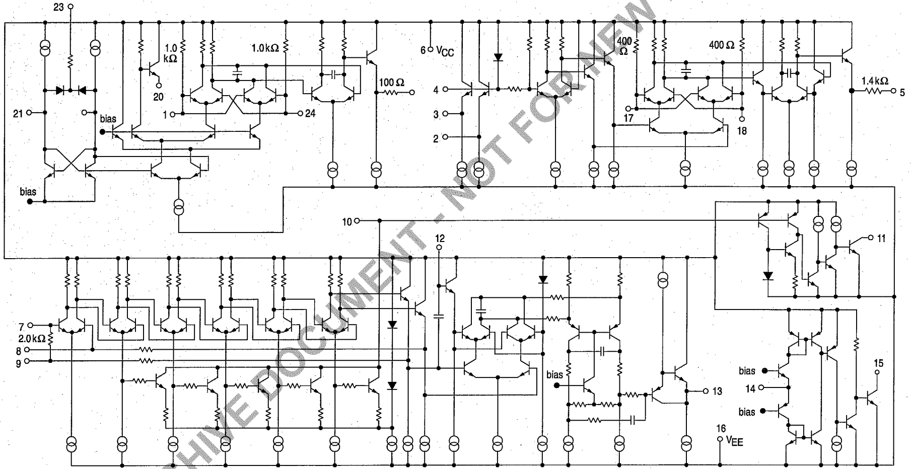
Figure 13. Representative Schematic Diagram
