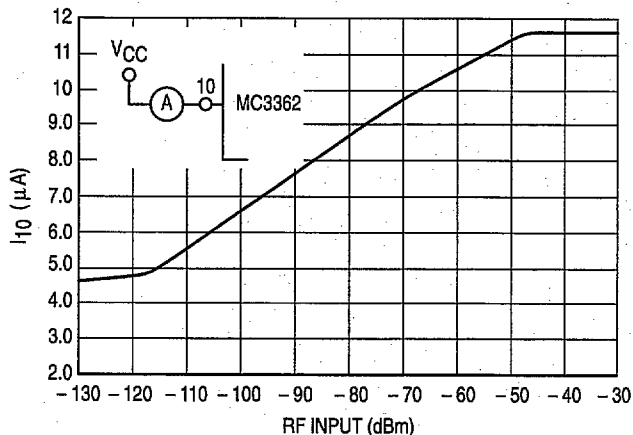
Figure 4. I_{10} Meter versus Input
