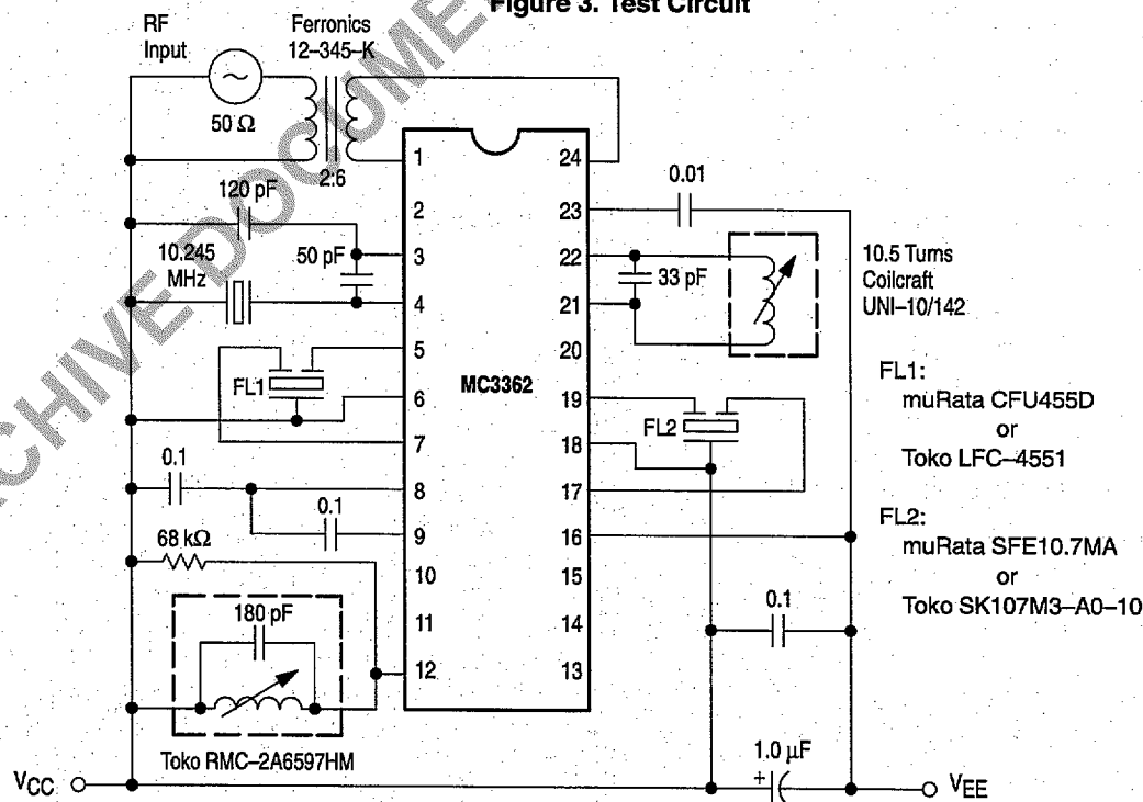
Figure 3. Test Circuit
