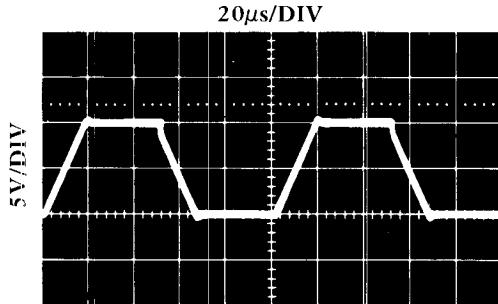
Figure 18. Output Waveform
