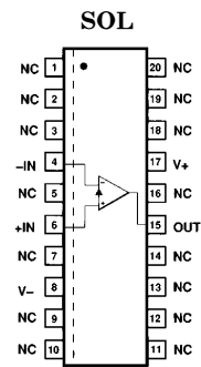
Top View
