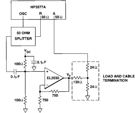
Figure 2. HDTV and Wideband Video Differential Gain and Phase Test Set-Up
