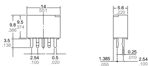
Self-clinching terminal
