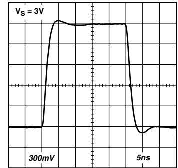
TPC 43. Large Signal Transient Response, G = 2
