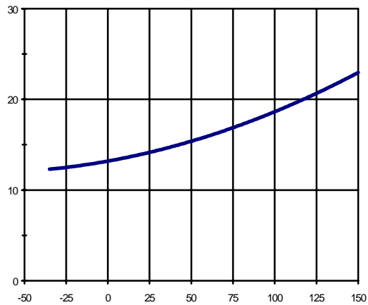
Figure 11 - R_{ds(on)} (mΩ) vs T_j ( ^\circ C )
