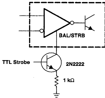
Figure 13. Strobing
