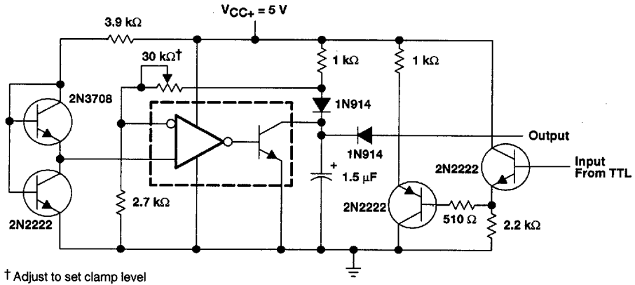
Figure 22. Precision Squarer
