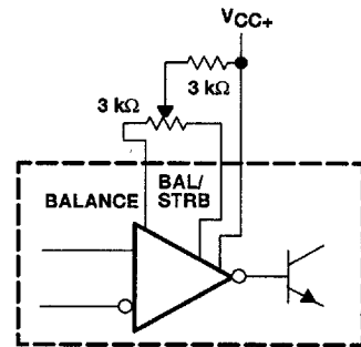
Figure 12. Offset Balancing
