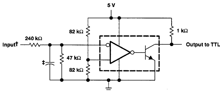
Figure 13. Strobing
