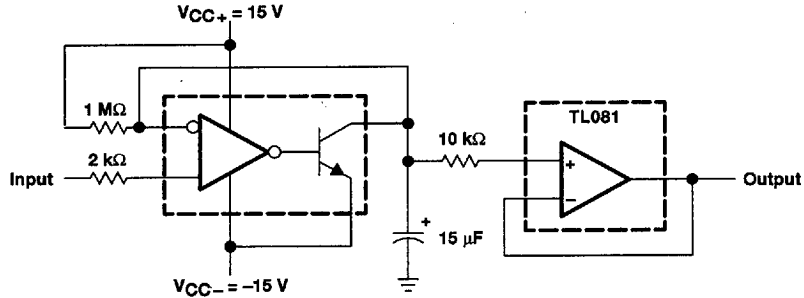
Figure 25. Negative-Peak Detector
