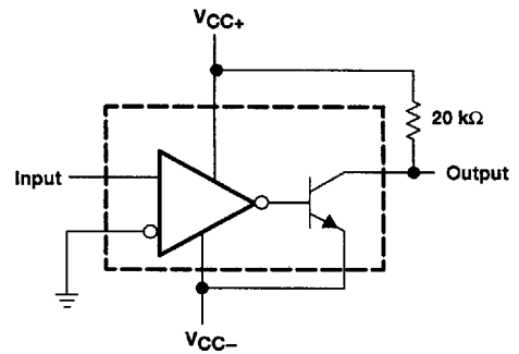
Figure 14. Zero-Crossing Detector
