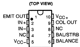
LM111 . . . U PACKAGE
