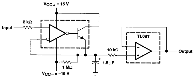
Figure 24. Positive-Peak Detector
