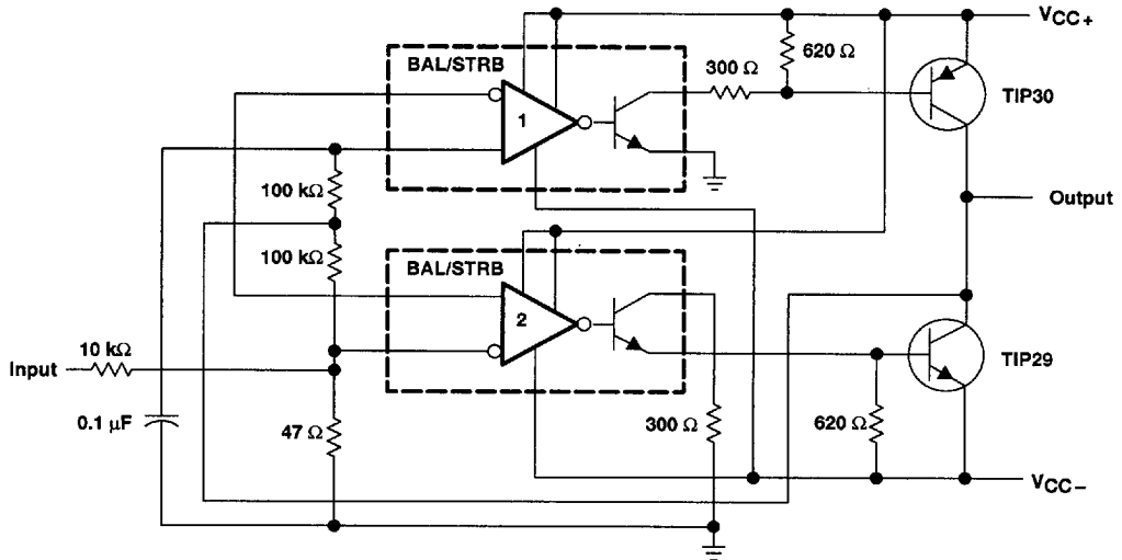
Figure 28. Switching Power Amplifier
