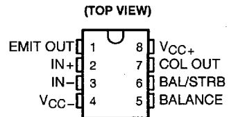
LM111 . . . U PACKAGE
