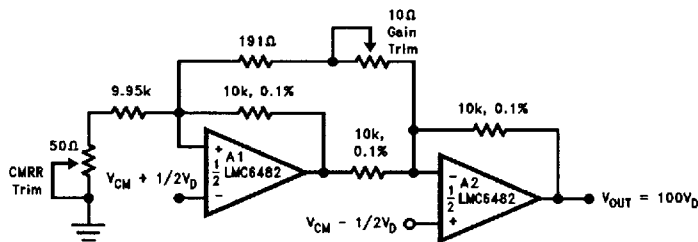
FIGURE 16. Low-Power Two-Op-Amp Instrumentation Amplifier
