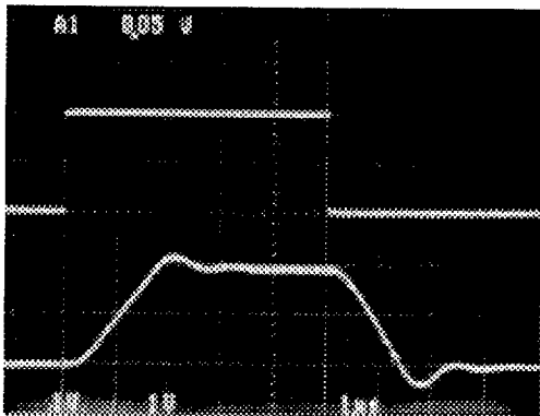
FIGURE 7. Pulse Response of LMC6482 Circuit in Figure 6
