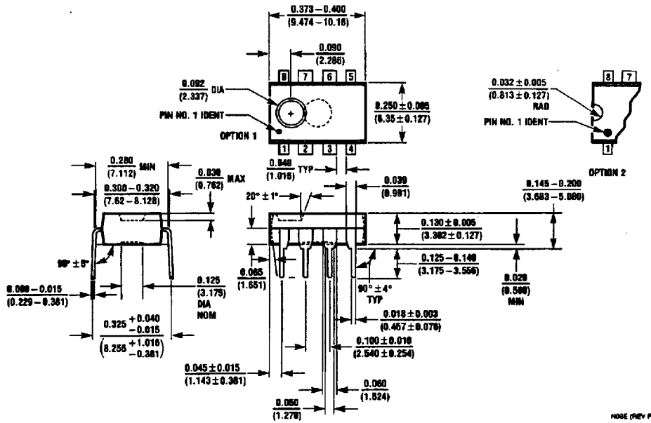
8-Pin Molded Dual-In-Line Package Order Package Number LMC6482AIN, LMC6482IN or LMC6482MN NS Package Number N08E
