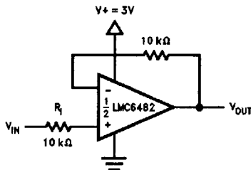
FIGURE 17. Half-Wave Rectifier with Input Current Protection (R 1 )
