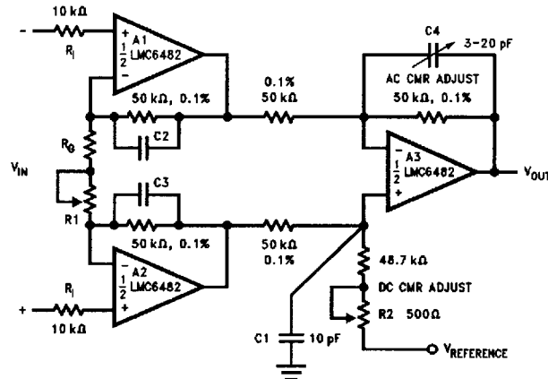
FIGURE 15. Low Power 3 Op-Amp Instrumentation Amplifier
