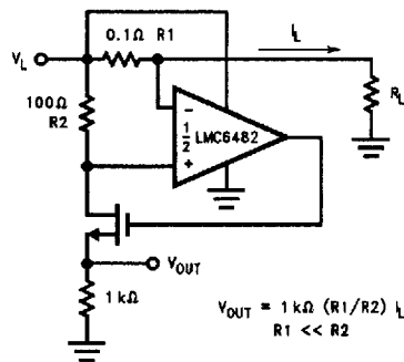
FIGURE 20. Positive Supply Current Sense
