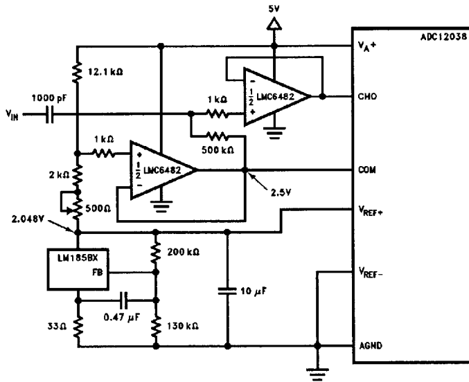
FIGURE 14. Operating from the same Supply Voltage, the LMC6482 buffers the ADC12038 maintaining excellent accuracy
