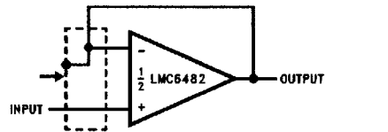
TL/H/11713-23 (c) Follower
