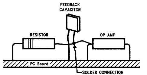
TL/H/11713-24 (Input pins are lifted out of PC board and soldered directly to components. All other pins connected to PC board.) FIGURE 11. Air Wiring
