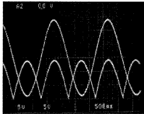
FIGURE 18A. Full Wave Rectifier Waveform
