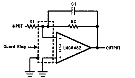
TL/H/11713-21 (a) Inverting Amplifier
