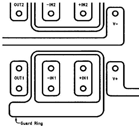
TL/H/11713-20 FIGURE 9. Example of Guard Ring in P.C. Board Layout
