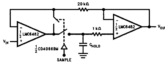
FIGURE 22. Rail-to-Rail Sample and Hold
