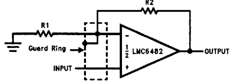
TL/H/11713-22 (b) Non-Inverting Amplifier
