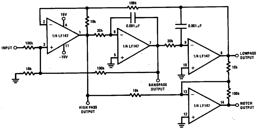
Universal State Variable Filter
