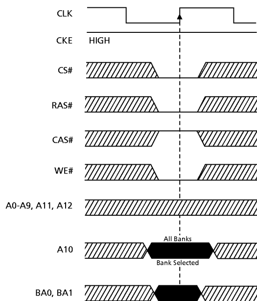
Figure 20 PRECHARGE Command
