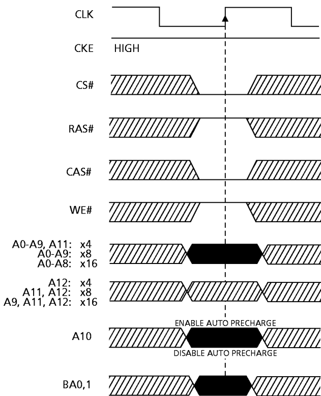
Figure 5 READ Command
