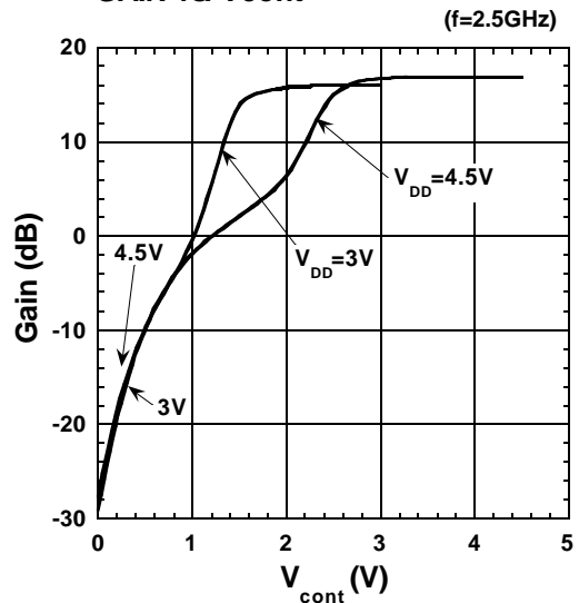
GAIN vs. V_{cont}
