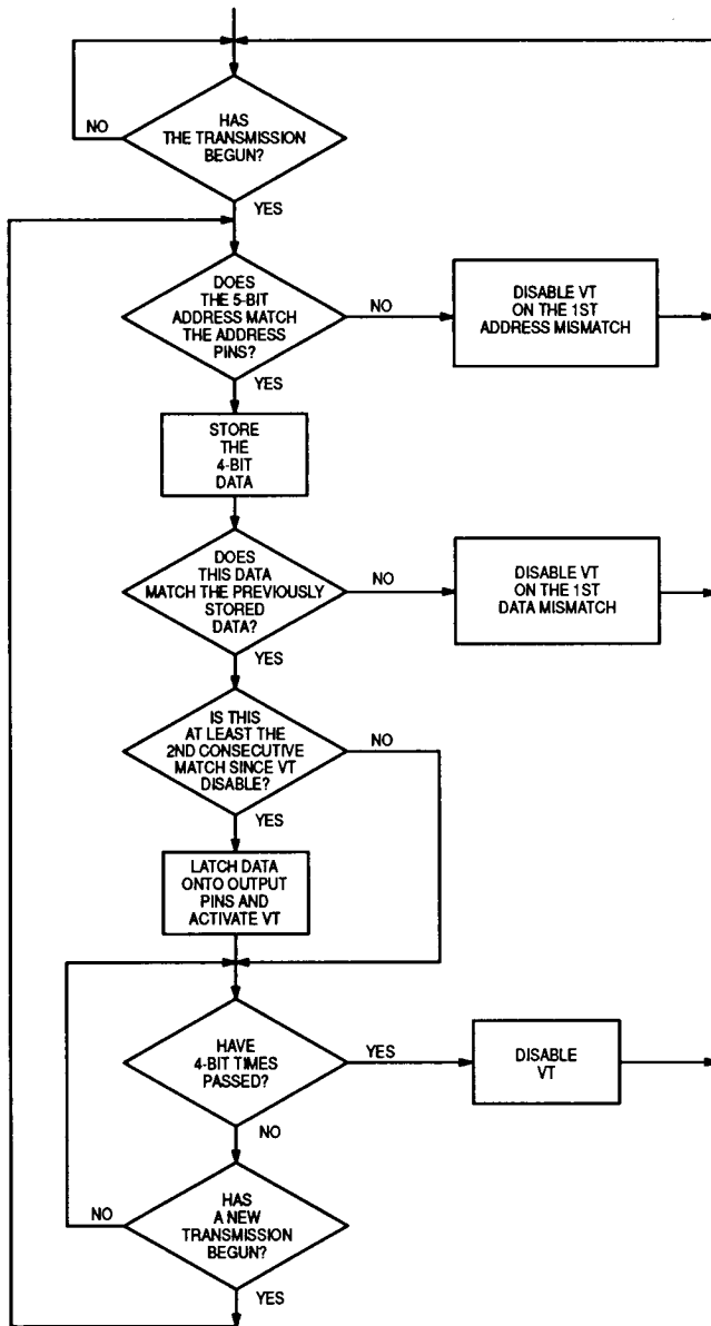
Figure 12. MC145027 Flowchart
