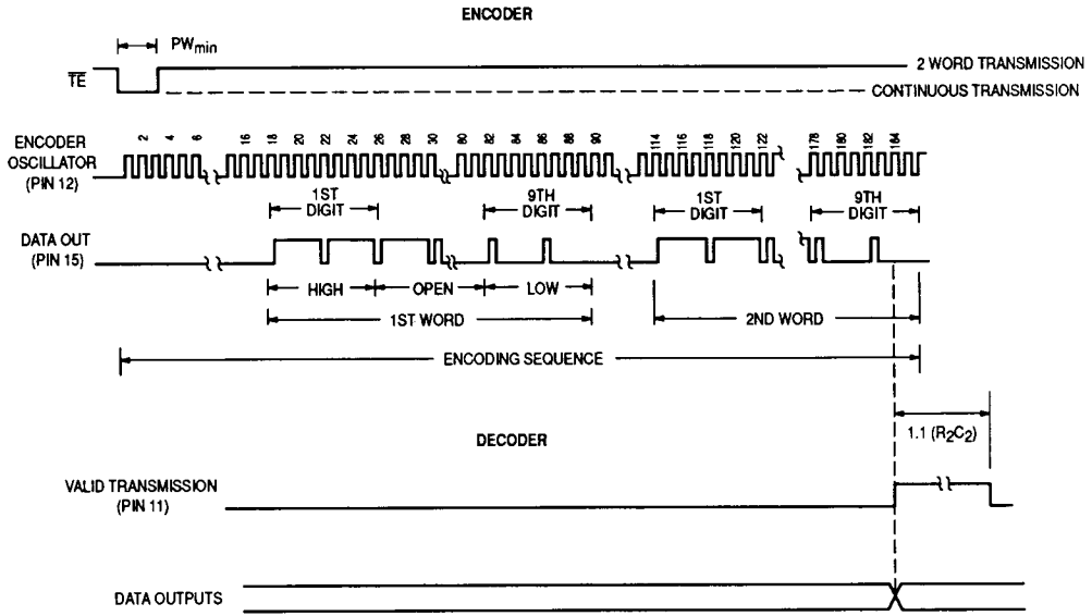
Figure 10. Timing Diagram
