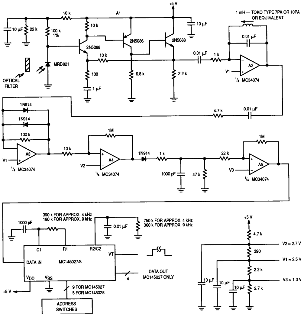
Figure 18. Infrared Receiver
