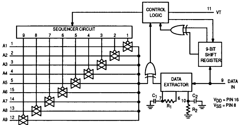
Figure 3. MC145028 Decoder Block Diagram
