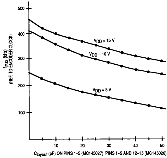
Figure 14. f_{max} vs C_{layout} — Decoders Only
