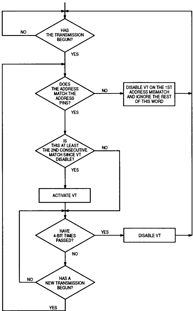
Figure 13. MC145028 Flowchart
