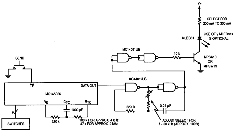
Figure 16. IRED Transmitter Using RC Oscillator to Generate Carrier Frequency
