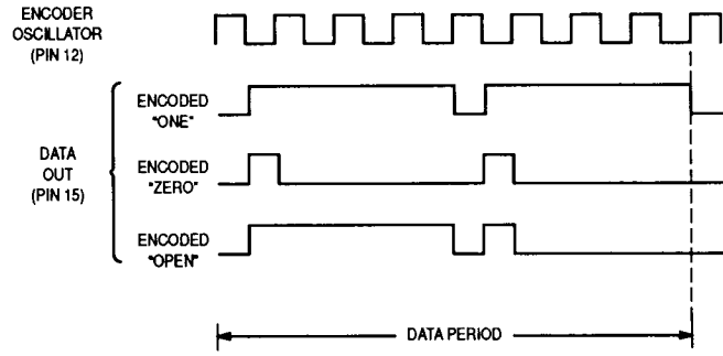
Figure 11. Encoder Data Waveforms
