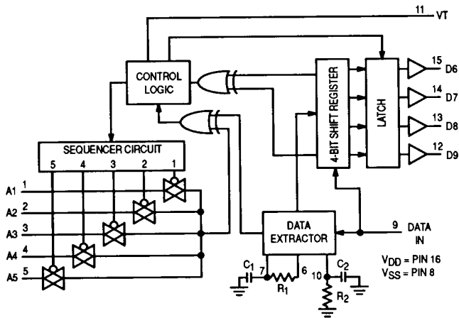
Figure 2. MC145027 Decoder Block Diagram
