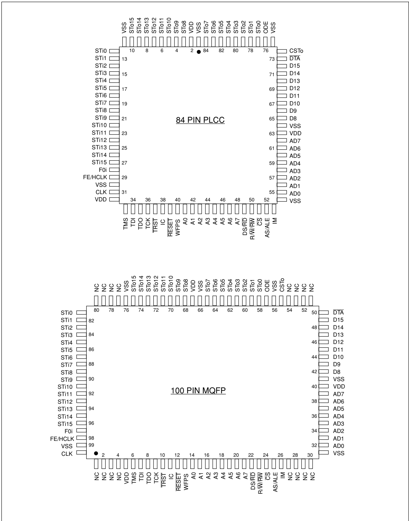
Figure 2 - Pin Connections
