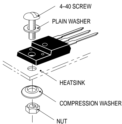
Figure 27a. Screw-Mounted
