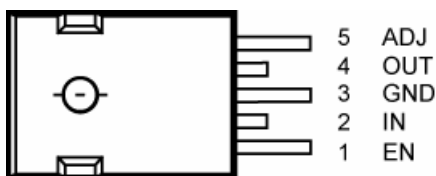
5-Pin TO-247 Adjustable Voltage (WT) MIC29752
