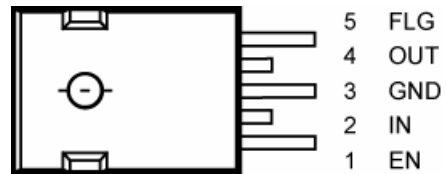
5-Pin TO-247 Fixed Voltage (WT) MIC29751
