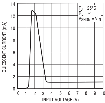
LT1963A-3.3 Quiescent Current
