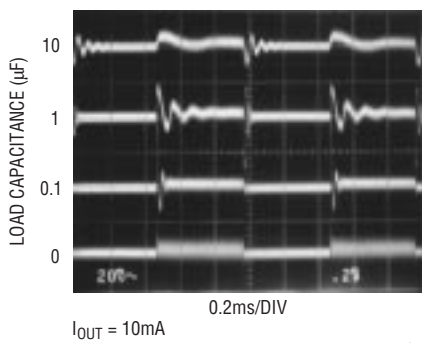
Transient Responses
