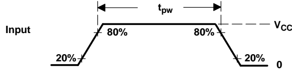
Figure 11. CMOS-Level Inputs
