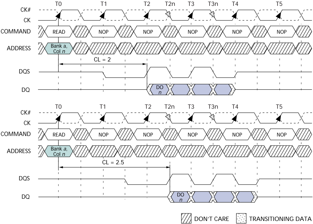
Figure 11: READ Burst
