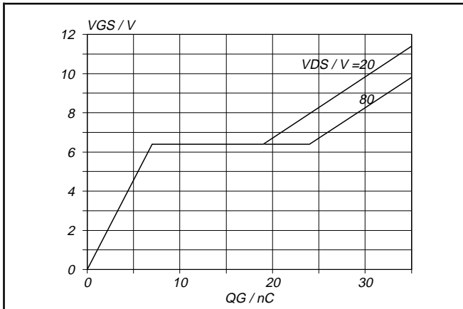
Fig.13. Typical turn-on gate-charge characteristics. V_{GS} = f(Q_G) ; conditions: I_D = 26 A; parameter V_{DS}
