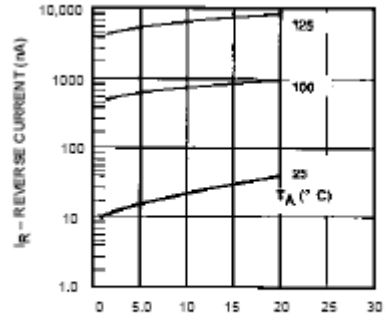
V_R – FORWARD VOLTAGE (V) (PULSED)
