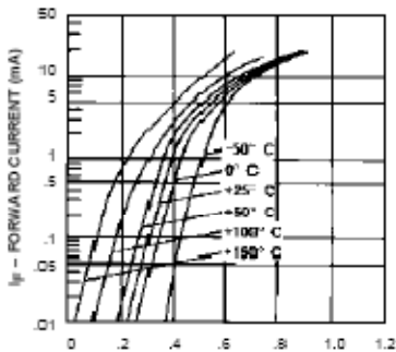
V_F – FORWARD VOLTAGE (V)
