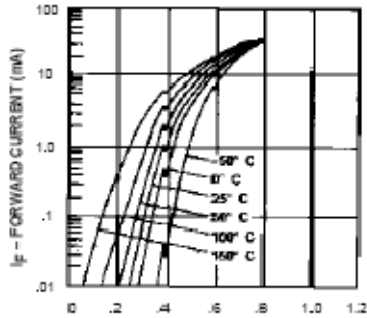
V_F – FORWARD VOLTAGE (V)
