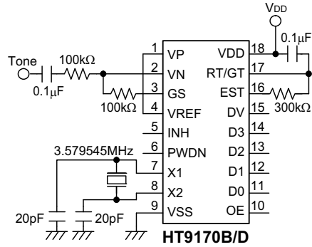
Figure 1. Test circuit
