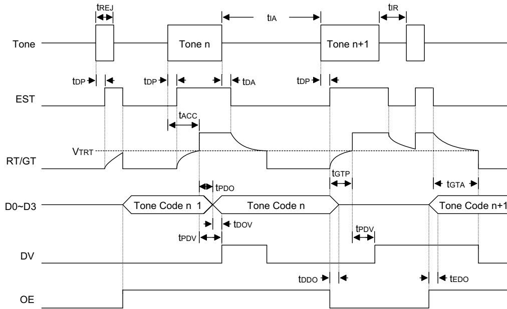
Figure 3. Steering timing
