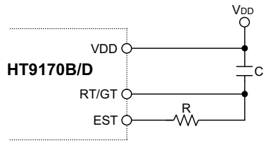
(a) Fundamental circuit:
