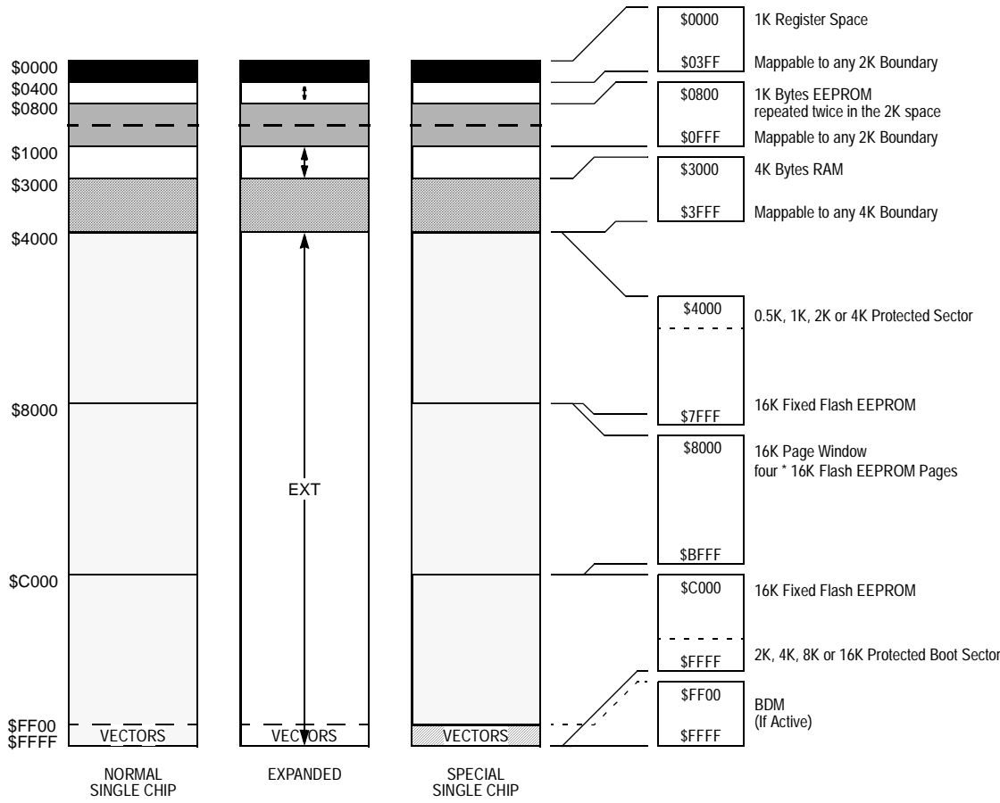
Figure 6 MC9S12Dx64 User Configurable Memory Map
