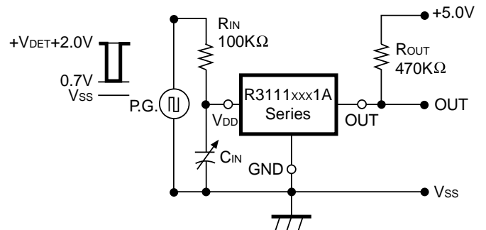
Figure 8. Output Delay Time Test Circuit (2)
