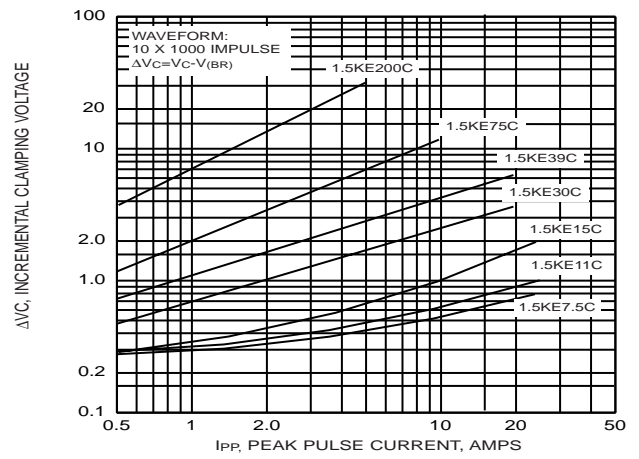
FIG. 10 - INCREMENTAL CLAMPING VOLTAGE CURVE BI-DIRECTIONAL
