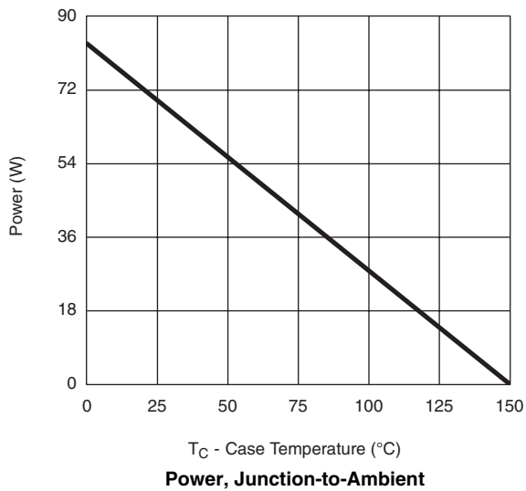
Power, Junction-to-Ambient
