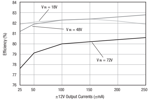
Efficiency vs. ±12V Output Loading (+5V output loaded @ 2.75A)
