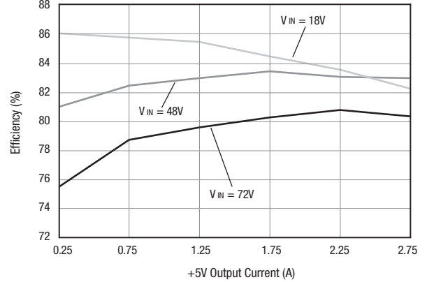
Efficiency vs. +5V Output Loading (±12V outputs loaded @ ±250mA)
