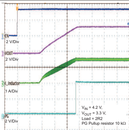
Figure 24. Start-up TPS62067 Into 2.2- \Omega Load With Power Good
