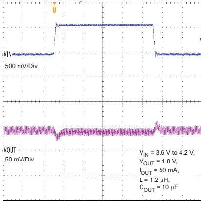
Figure 22. Line Transient PFM Mode
