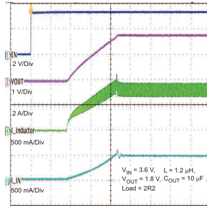
Figure 23. Startup Into Load – V_{OUT} = 1.8 \text{ V}
