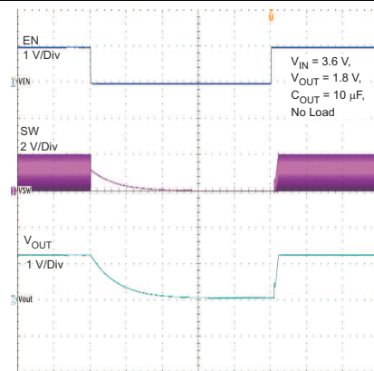
Figure 25. Output Discharge
