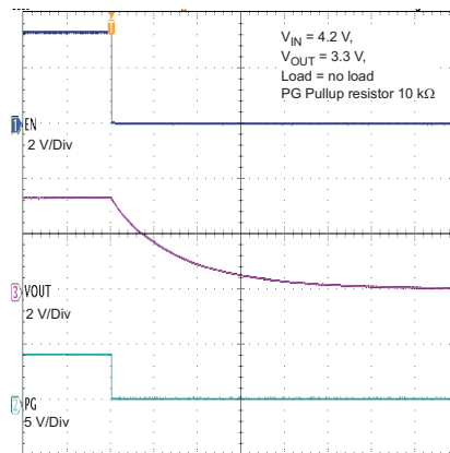
Figure 26. Shutdown TPS62067
