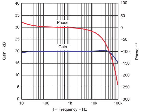
Gain = 20 dB V_{CC} = 12\text{ V} Z_L = 8\ \Omega + 66\ \mu\text{H} C_1 = \mu\text{F} V_1 = 0.1\text{ V}_{\text{RMS}} Filter = Audio Precision AUX-0225
