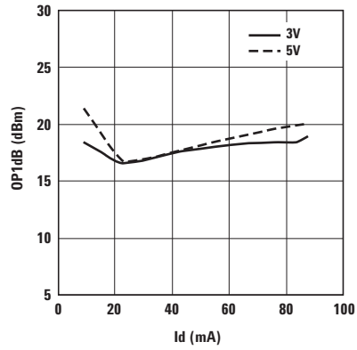
Figure 27. OP1dB vs. Id (500 MHz).
