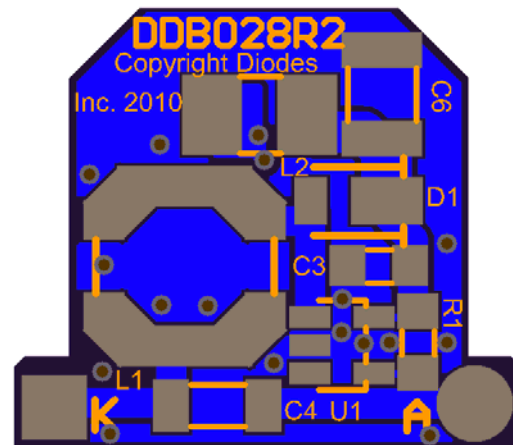
Figure 38. Bottom Layer
