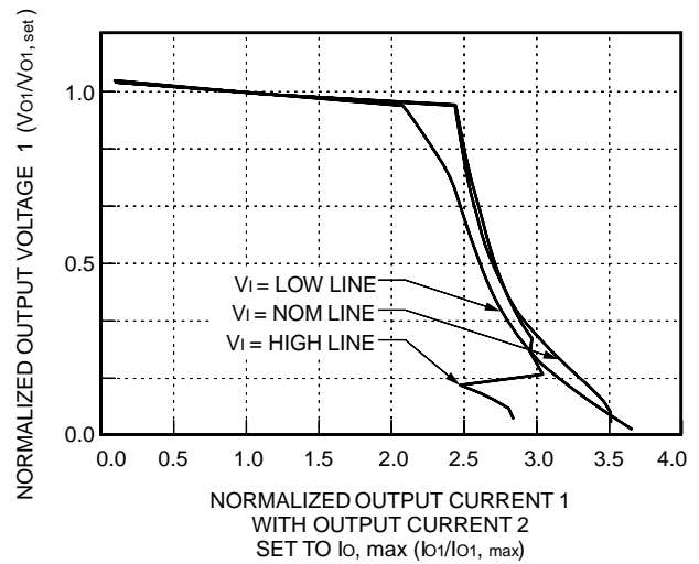
Note: Output2 has characteristics similar to output1 when output1 is set to I_{o, \max} .
