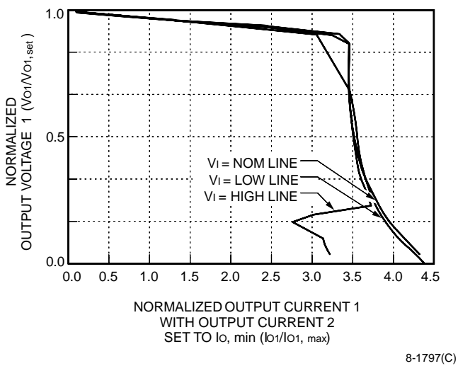
Note: Output2 has characteristics similar to output1 when output1 is set to I_{o, \min} .
