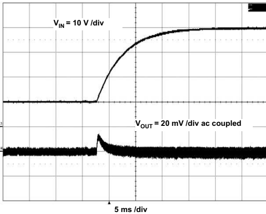
Figure 29. Line Transient
