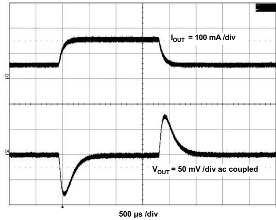
Figure 28. Load Transient
