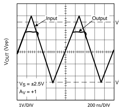
Figure 60. Input and Output Shown with CMVR Exceeded
