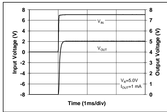
FIGURE 2-36: Startup Response.
