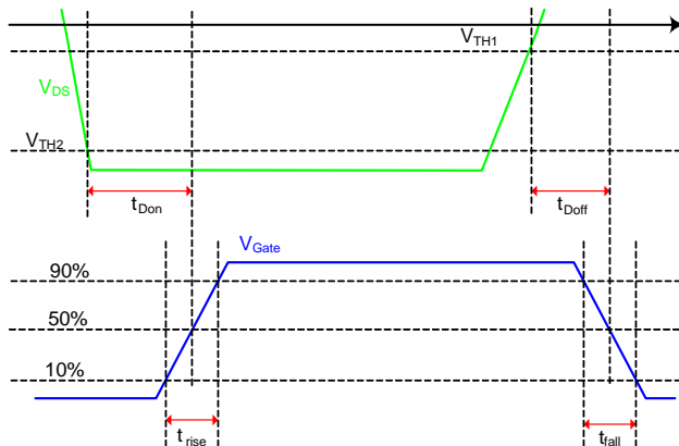
Figure 12: Timing waveform
