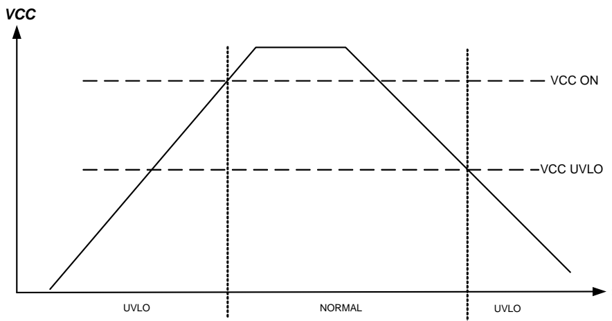
Figure 11: Vcc UVLO
