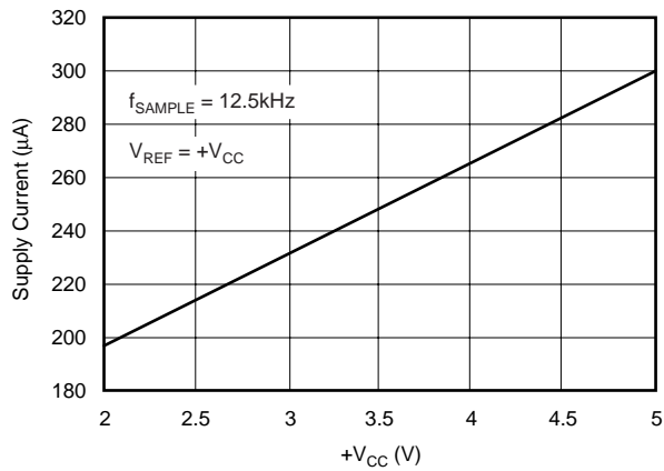
SUPPLY CURRENT vs +V CC
