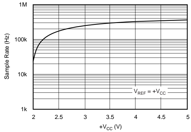
MAXIMUM SAMPLE RATE vs +V CC
