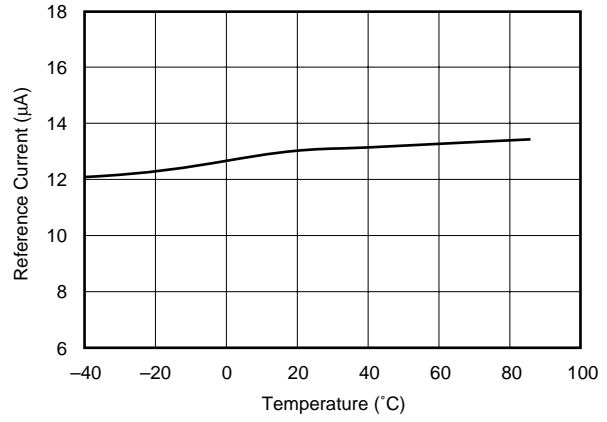
REFERENCE CURRENT vs TEMPERATURE
