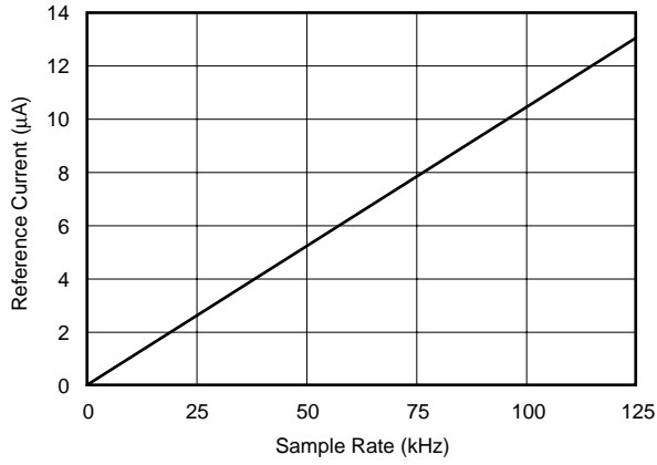
REFERENCE CURRENT vs SAMPLE RATE
