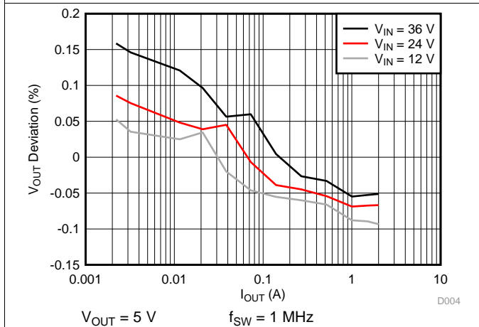
Figure 5. Load Regulation
