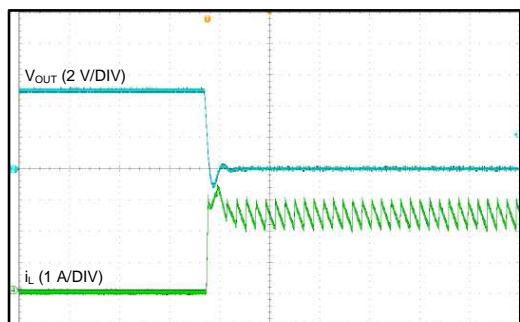
Figure 26. CCM Mode
