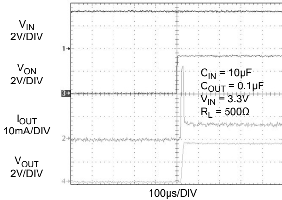
Figure 15. T_{ON} Response
