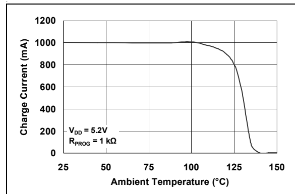
FIGURE 4-3: Thermal Regulation
