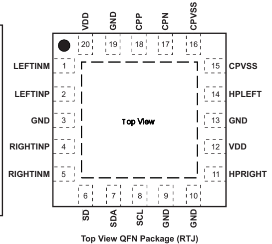
Top View QFN Package (RTJ)
