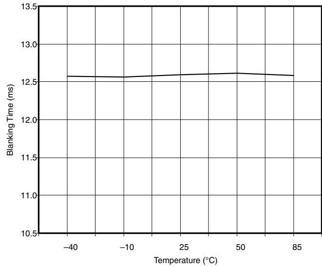
Figure 17. t_{BLANK} vs Temperature ( V_{IN} = 3.3 \text{ V} )
