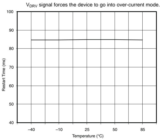
Figure 18. t_{RESTART} vs Temperature ( V_{IN} = 3.3 \text{ V} )
