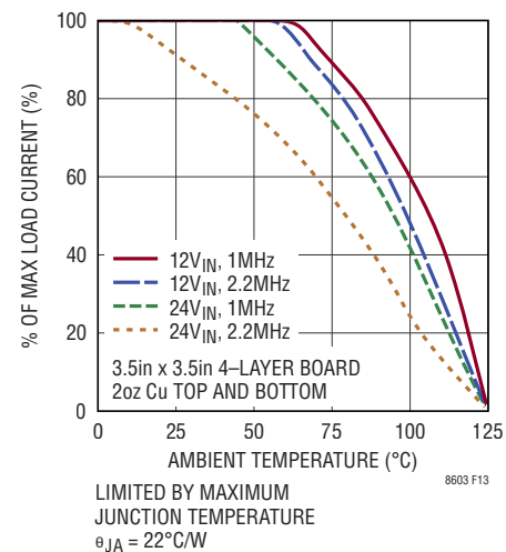
Figure 13. Thermal Derating, E- and I-Grade
