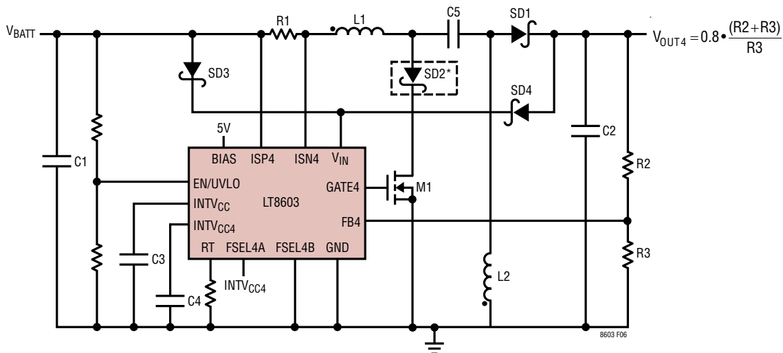
Figure 6. Channel 4 in SEPIC Configuration
