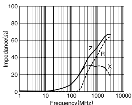
MMZ1608D100C
